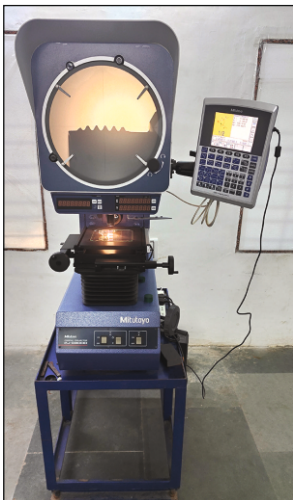
Precision Profile Projector
